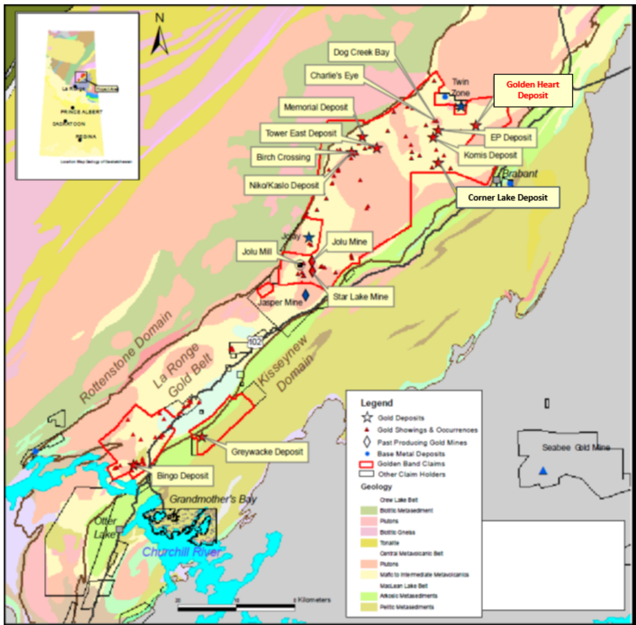
FIGURE 7.1 REGIONAL GEOLOGY
